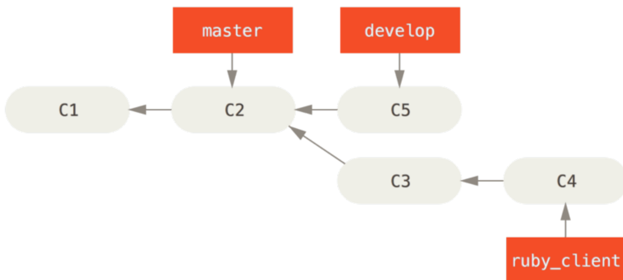
Figure 75. Before a topic branch merge.
